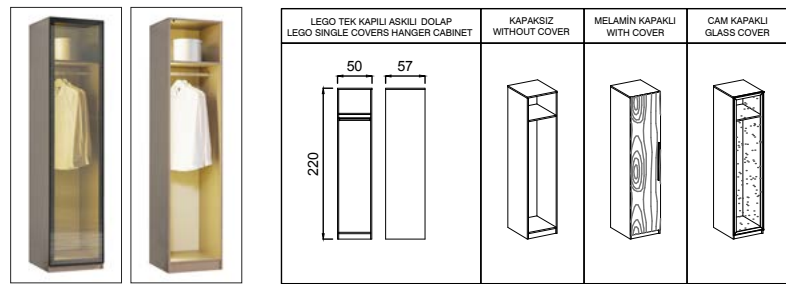
LEGO SINGLE COVERS HANGER CABINET
