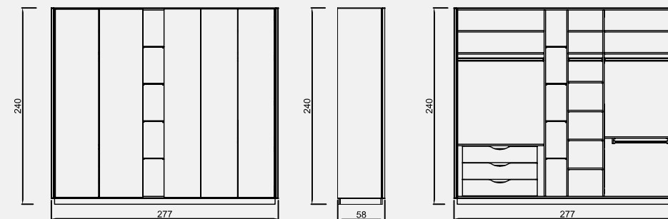
WARDROBE ATLANTIS
